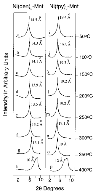
Fig. 4. X-ray diffraction patterns and basal spacing ( d_{001} ) of oriented samples of intercalated [\text{Ni}(\text{den})_2] -Mnt (a–h) and [\text{Ni}(\text{tpy})_2] -Mnt (i–p) composites heated at different temperature (50–400°C) for 1 h in air atmosphere.
